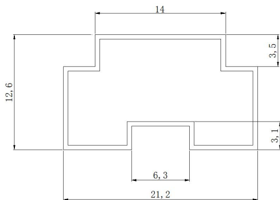
Fig.8 Section schematic diagram
