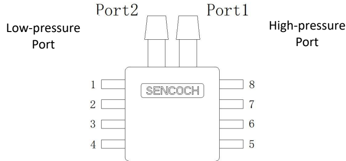
Fig.2 Pin configuration diagram
