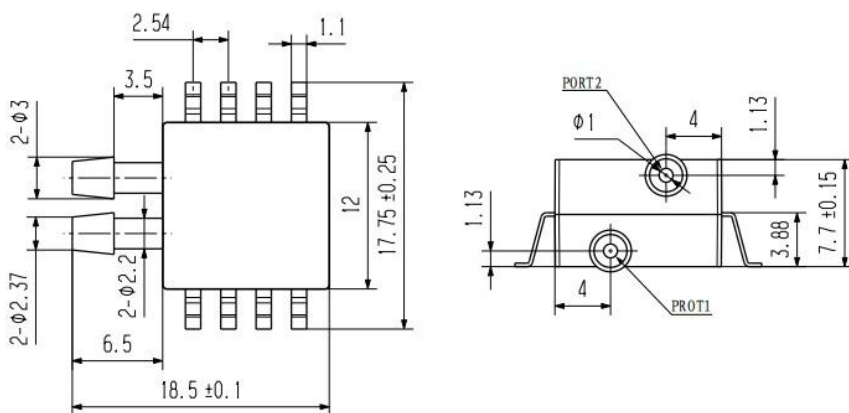
Fig.6 Sensor Dimensions
