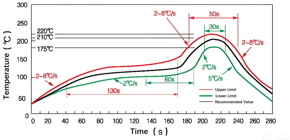
Fig.8 Remelting temperature setting conditions
