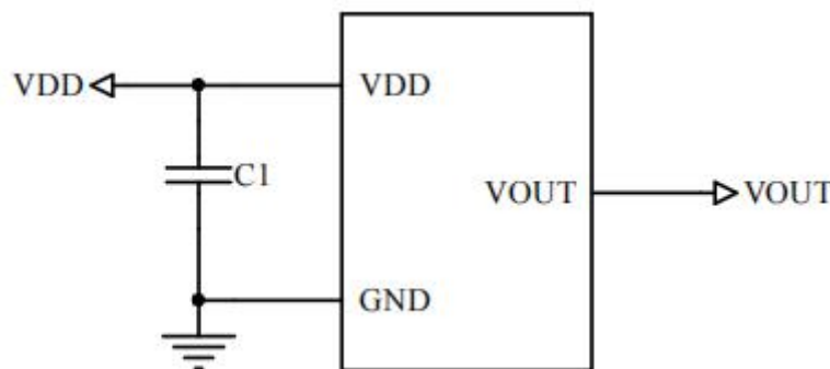
Fig.5 Application circuit
