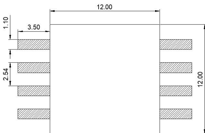
Fig.7 Recommended Footprint
