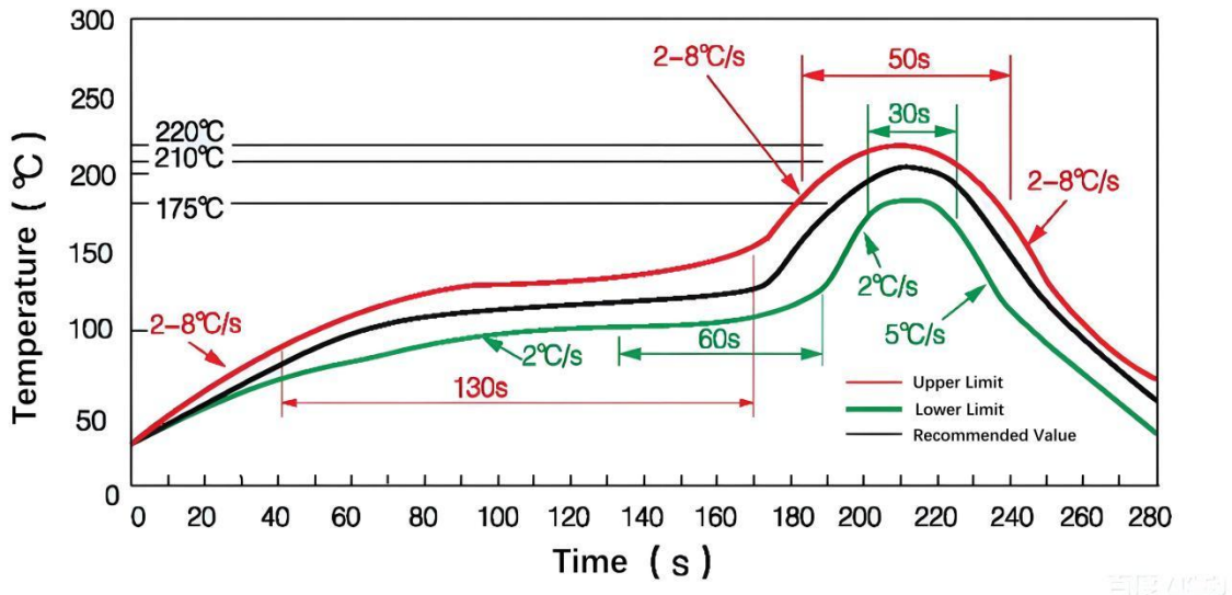
Fig.10 Remelting temperature setting conditions
