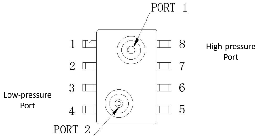
Fig.2 Pin configuration diagram
