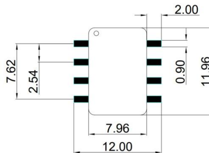
Fig.9 Recommended footprint
