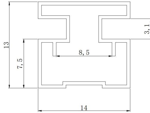
Fig.11 Section schematic diagram
