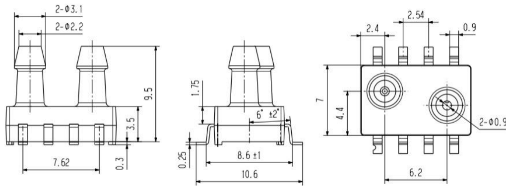
Fig.8 Product dimensions
