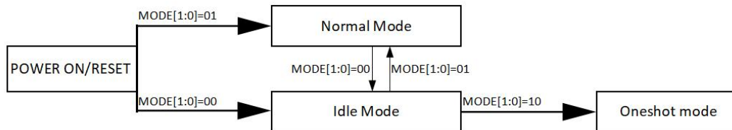
Fig.7 Working Mode
