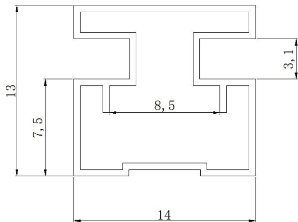
Fig.8 Section schematic diagram
