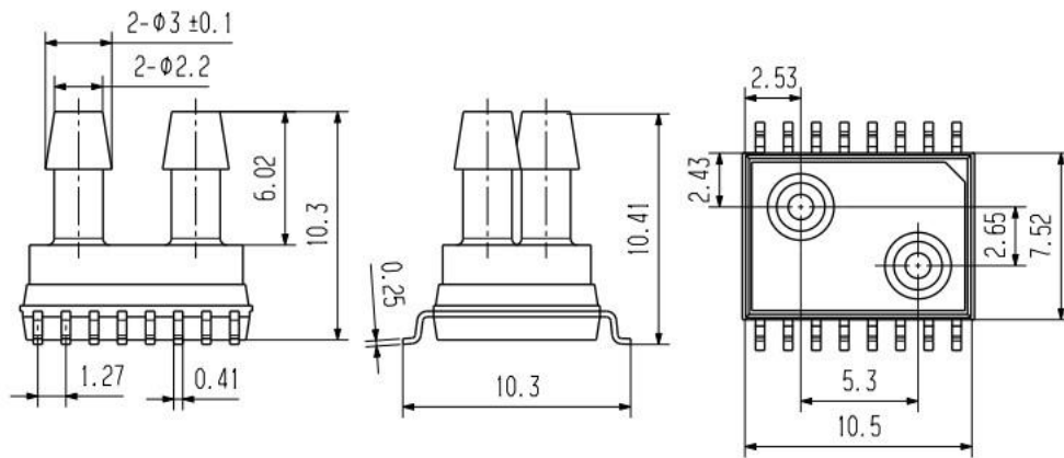
Fig.6 Sensor Dimensions
