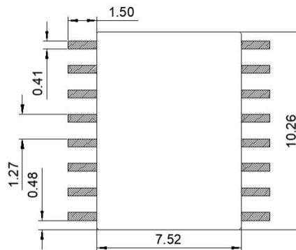
Fig.7 Recommended Footprint
