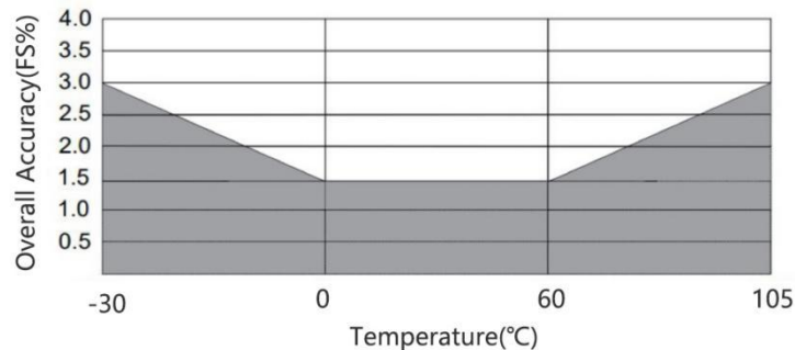
Fig.4 Relationship between overall accuracy and temperature
