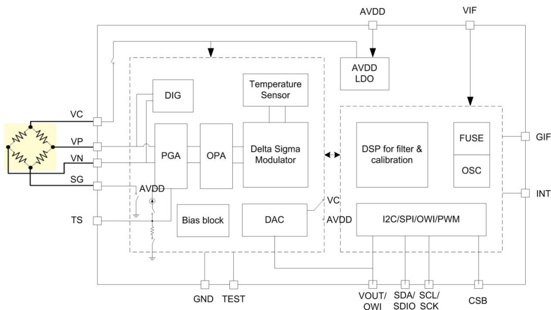
Fig.1 Block Diagram
