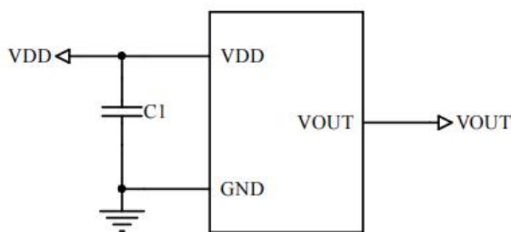
Fig.5 Application circuit
