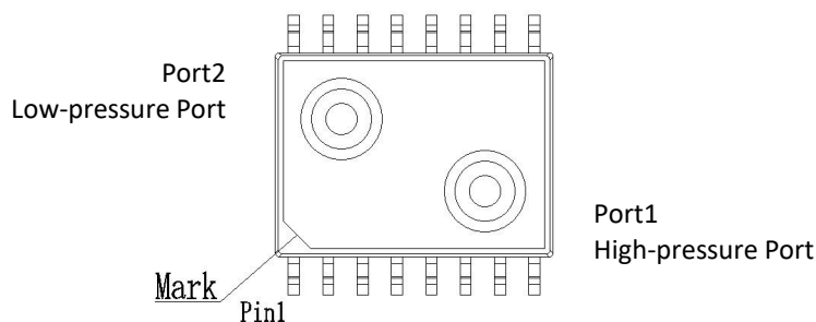
Fig.2 Pin configuration diagram
