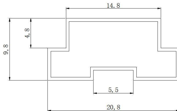
Fig.8 Section schematic diagram
