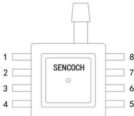
Fig.2 Pin configuration diagram
