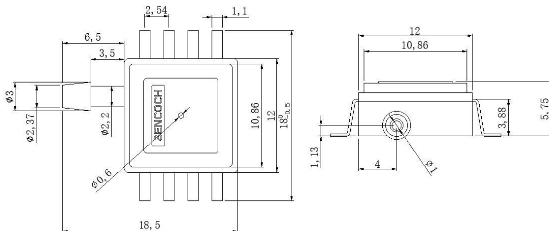
Fig.6 Sensor Dimensions
