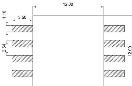
Fig.7 Recommended Footprint
