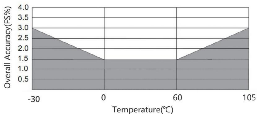
Fig.4 Relationship between overall accuracy and temperature
