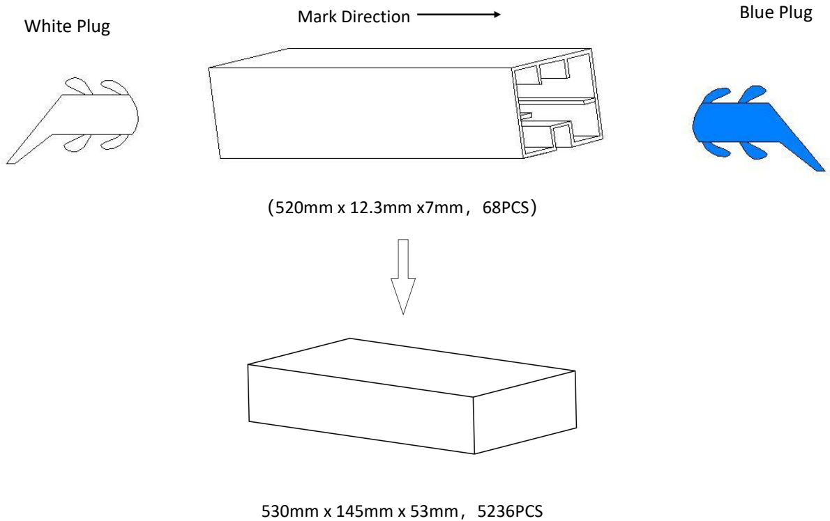
Fig.10 Outer Packing
