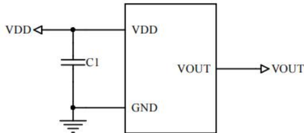
Fig.5 Application circuit
