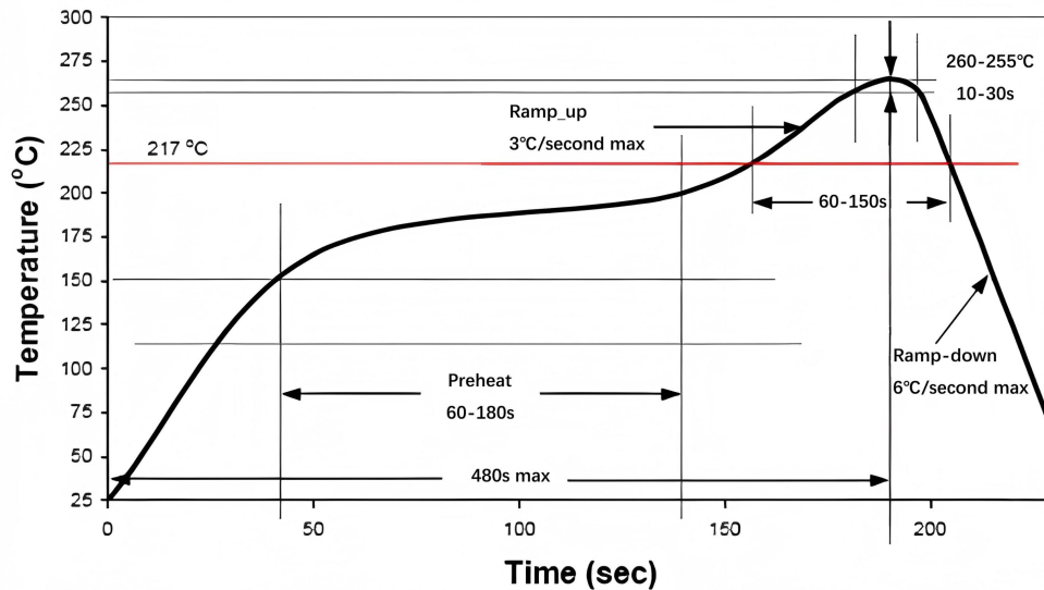
Fig.8 Reflow soldering
