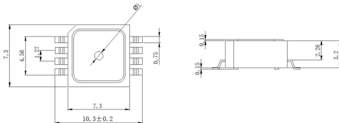
Fig.6 Sensor Dimensions
