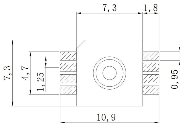
Fig.7 Recommended Footprint
