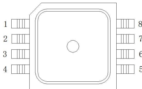
Fig.2 Pin Diagram
