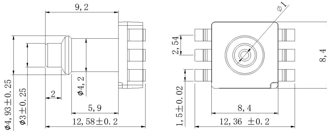
Fig.8 Product dimensions
