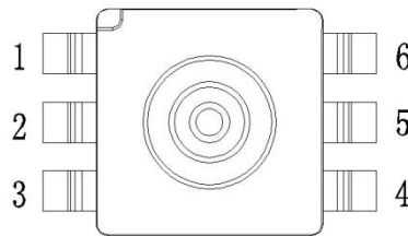
Fig.2 Pin configuration diagram
