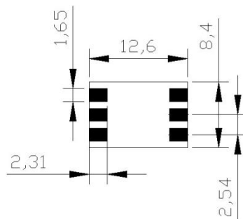
Fig.9 Recommended footprint
