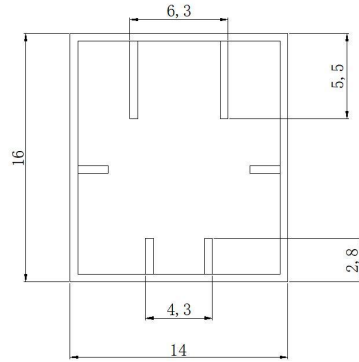
Fig.11 Section schematic diagram
