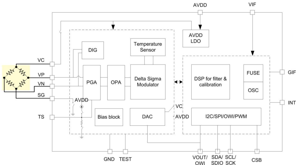
Fig.1 Block Diagram
