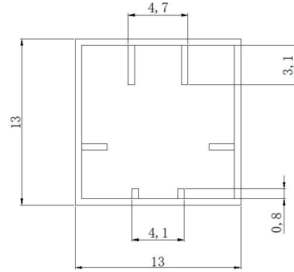
Fig.8 Section schematic diagram
