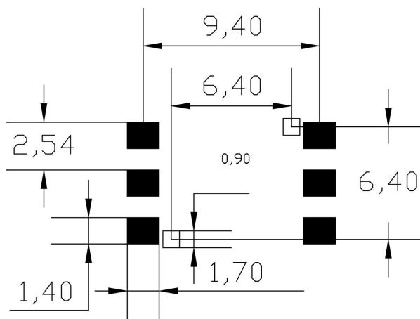
Fig.7 Recommended Footprint
