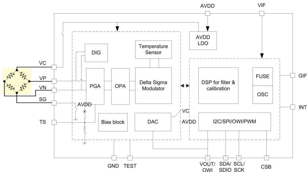
Fig.1 Block Diagram
