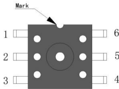
Fig.2 Pin configuration diagram
