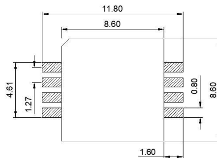
Fig.7 Recommended Footprint
