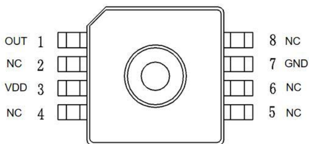
Fig.2 Pin Diagram
