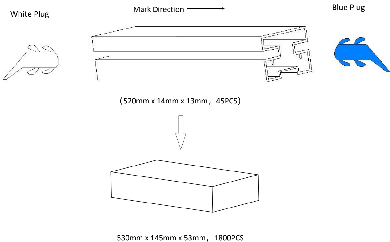
Fig.10 Outer Packing
