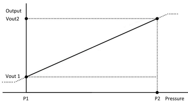
Fig.3 Pressure sensor transfer characteristic curve
