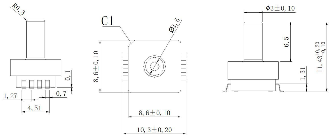
Fig.6 Sensor Dimensions
