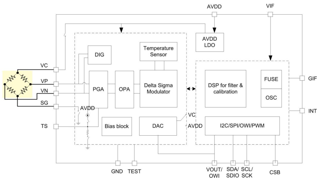
Fig.1 Block Diagram
