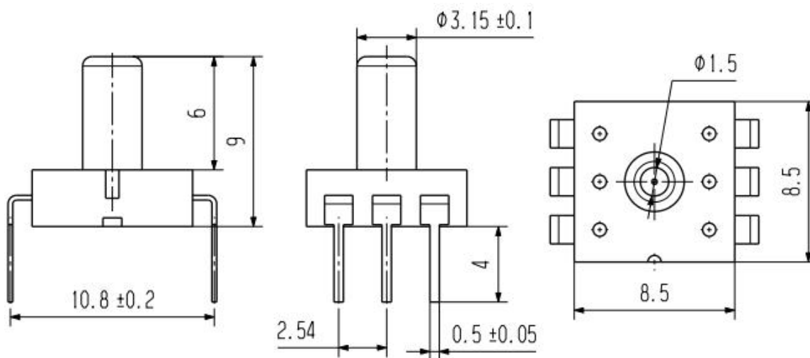
Fig.6 Sensor Dimensions
