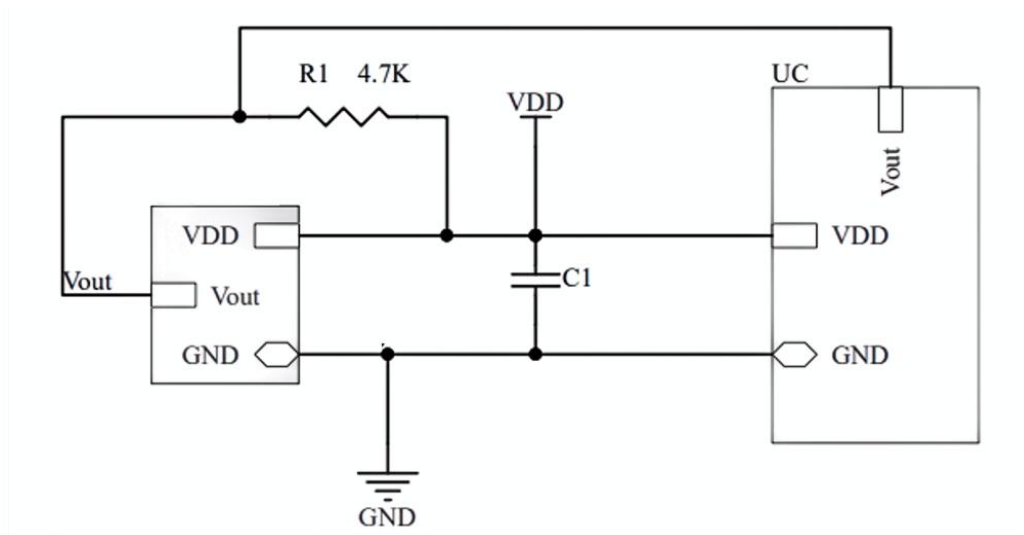
Fig.5 Application Circuit
