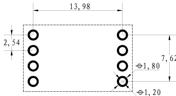
Fig.7 Recommended footprint
