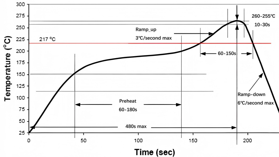
Fig.8 Reflow soldering
