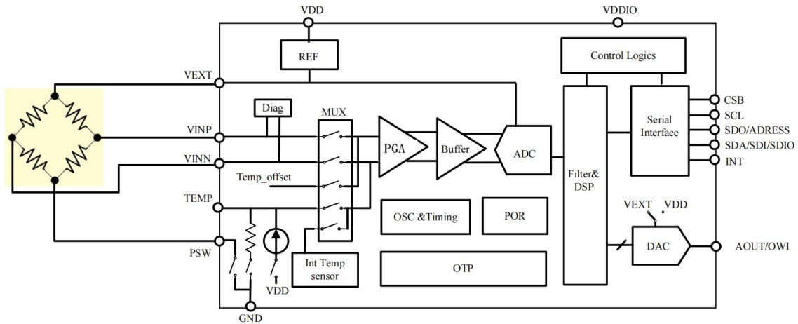
Fig.1 Block diagram
