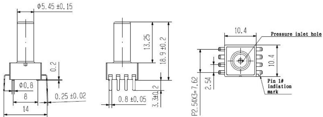
Fig.6 Sensor dimensions
