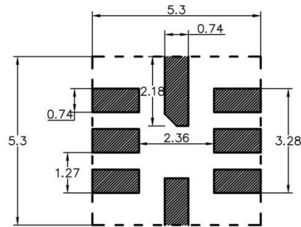
Fig.6 Footprint dimensions
