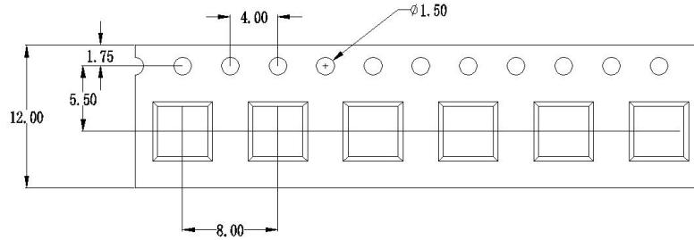
Fig.8 Tape
