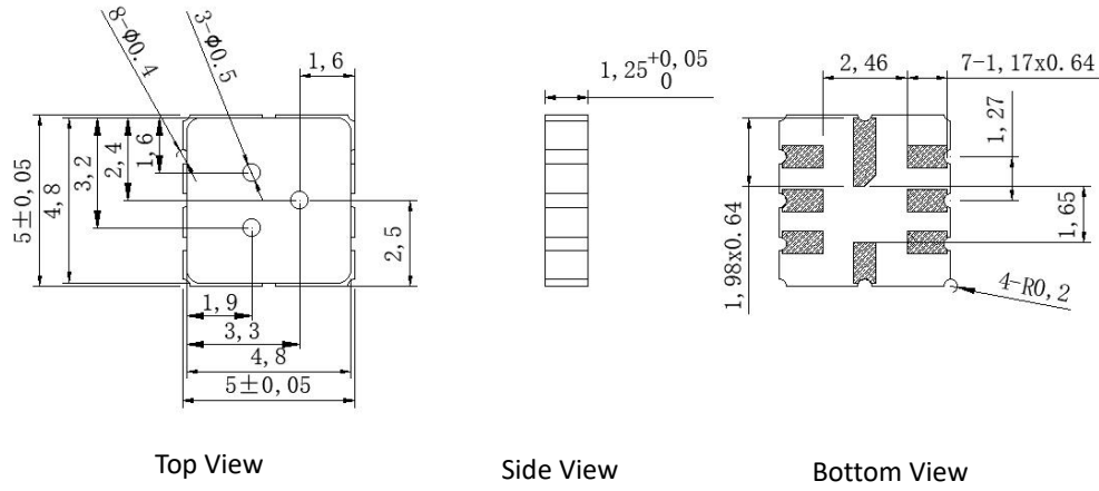
Fig.5 Product dimensions
