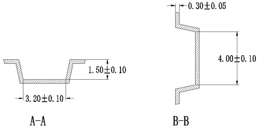
Fig.10 Detail of the carrier pocket
