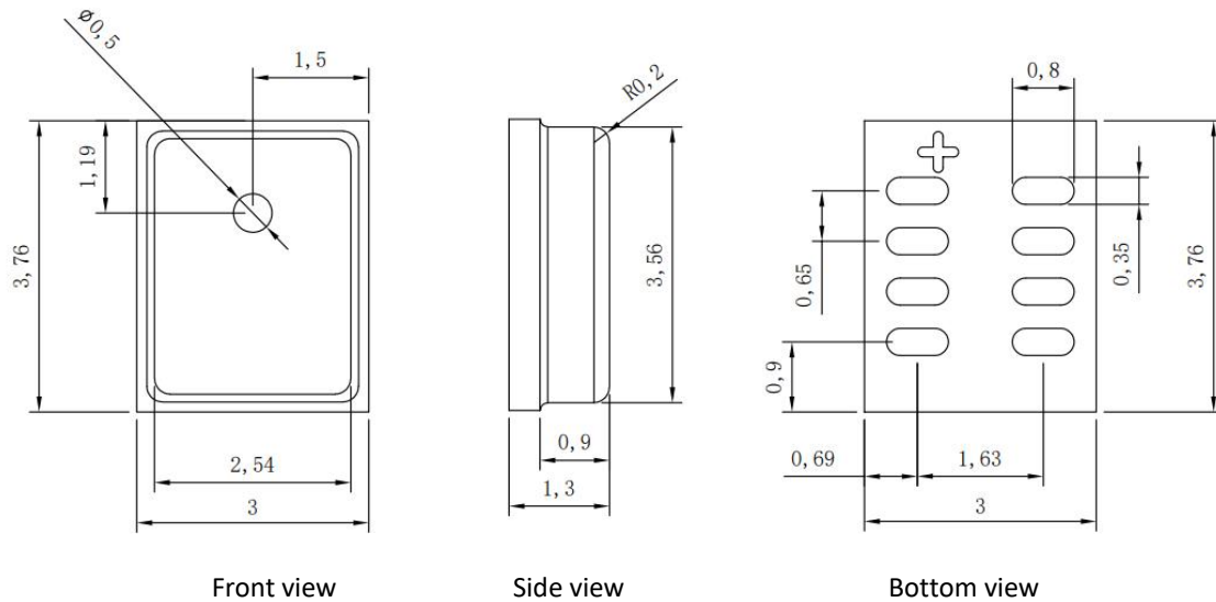
Fig.6 Sensor Dimensions
