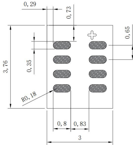
Fig.7 Recommended Footprint
