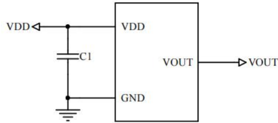
Fig.5 Application circuit
