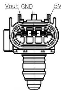
Fig.1 Pin diagram
