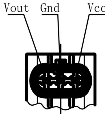
Fig.1 Pin diagram
