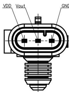
Fig.1 Pin diagram
