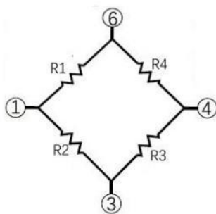
Fig.2 Schematic diagram
