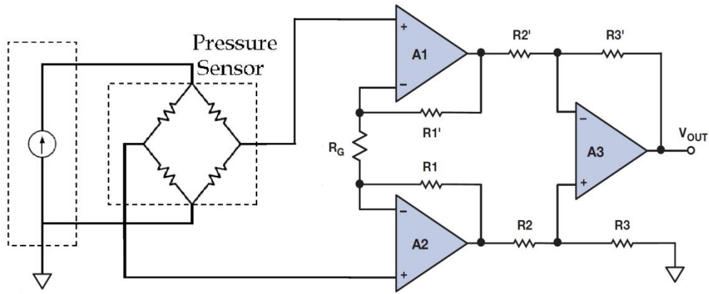
Fig.5 Amplifier circuit example
