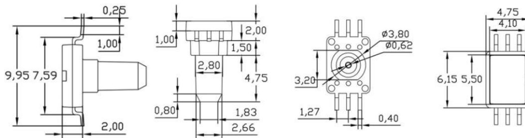
Fig.3 Appearance structure
