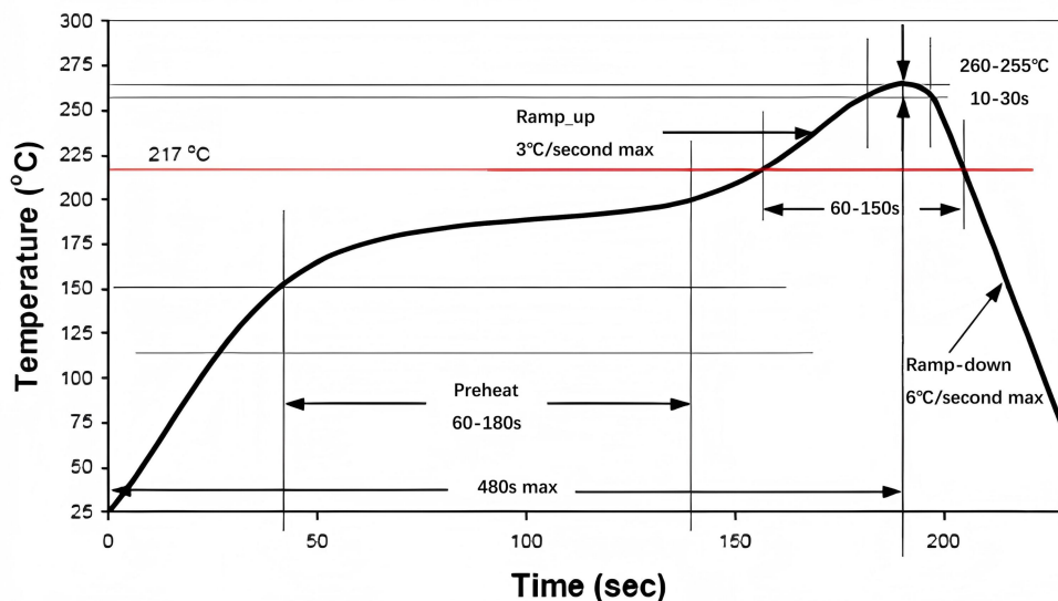
Fig.4 Reflow soldering temperature setting conditions
