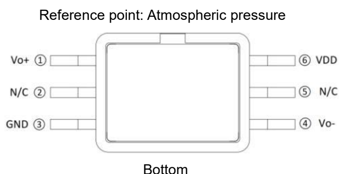
Fig.1 Pin Definition
