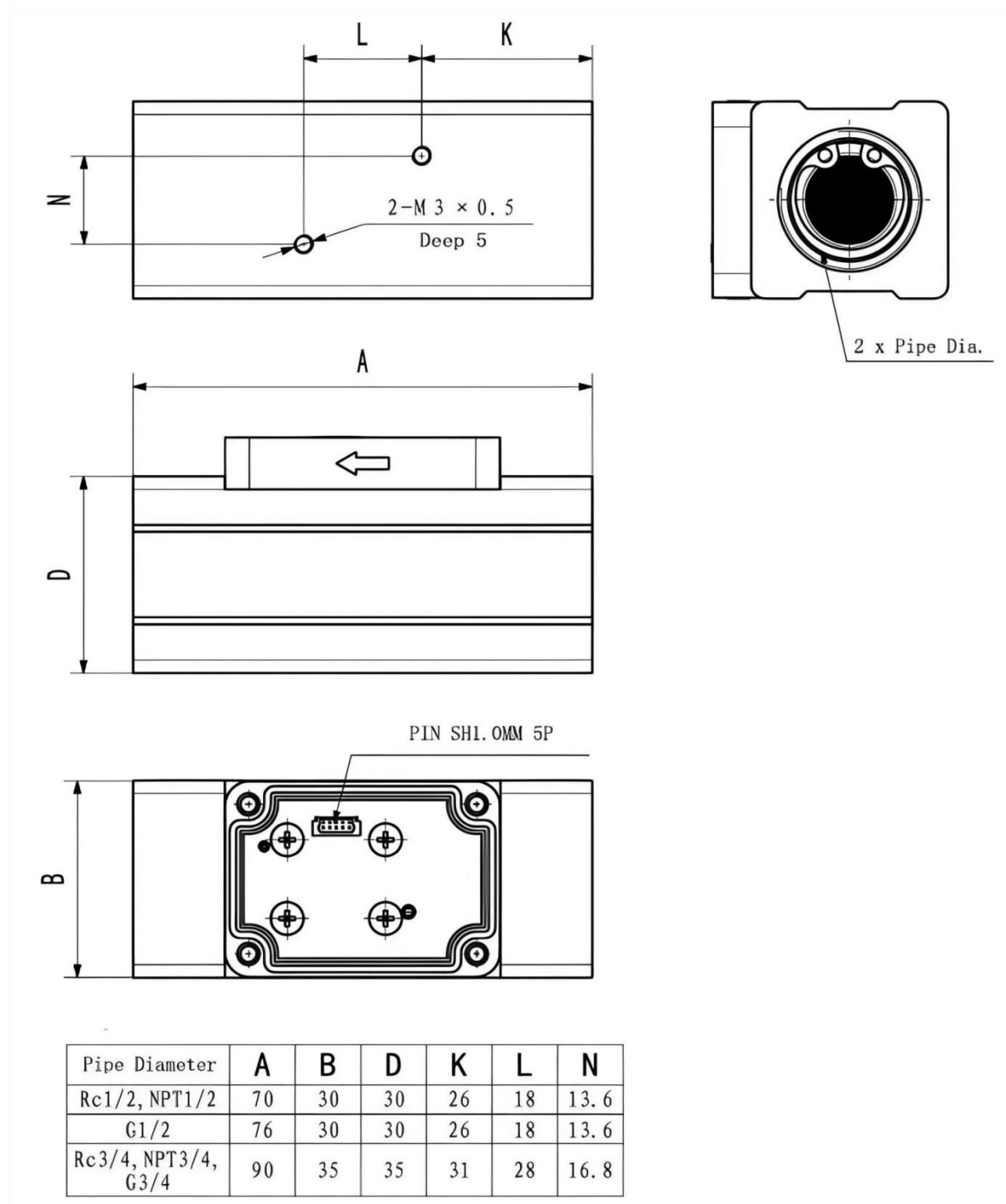
Figure 1 Sensor dimensions(without cover)
