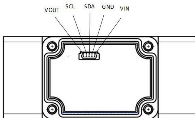
Figure 2. 1.0 mm 5 Pin Vertical Mounting Connector
